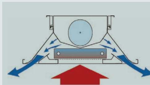
Chilled beams generate low velocity air diffusion for user comfort.
