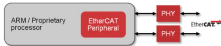
Figure 6. Integrated EtherCAT with processor
