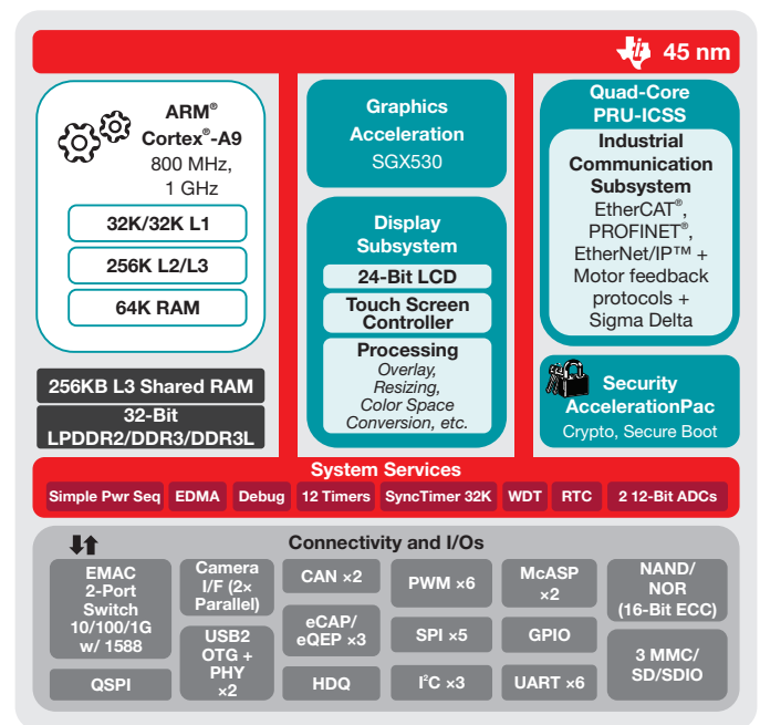
Figure 9. AM437x Sitara processor block diagram
