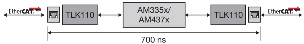
Figure 12. EtherCAT RX-TX latency
