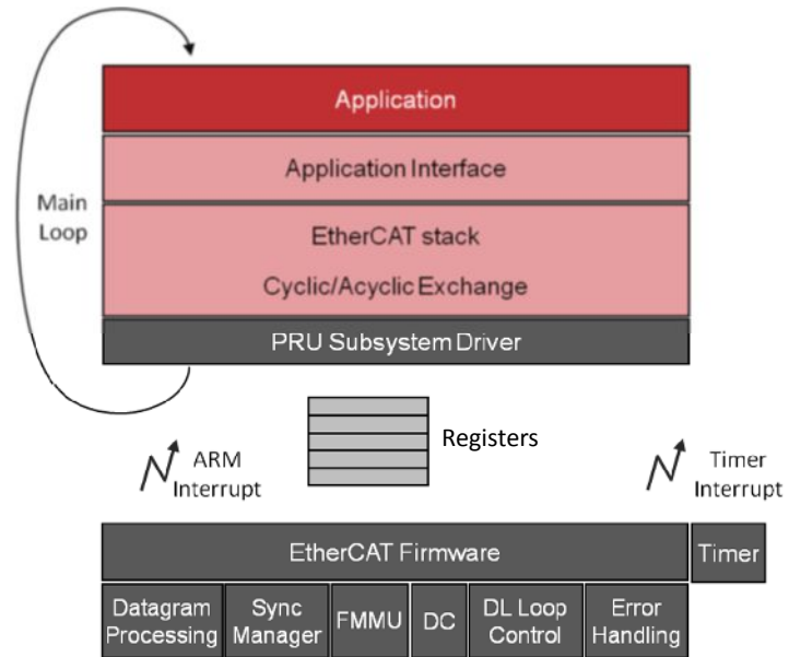
Figure 13. EtherCAT software integration
