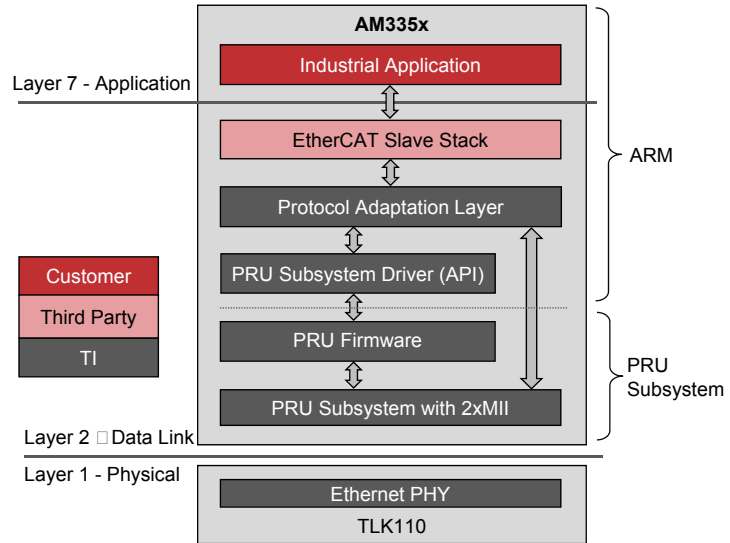
Figure 10. Software architecture for EtherCAT slave
