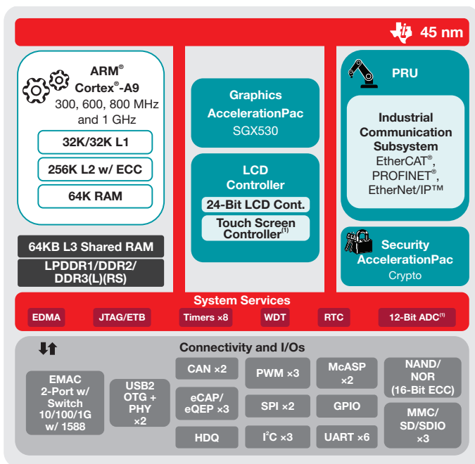
Figure 8. AM335x processor block diagram
