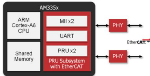
Figure 7. EtherCAT slave on TI Sitara AM335x / AM437x processors
