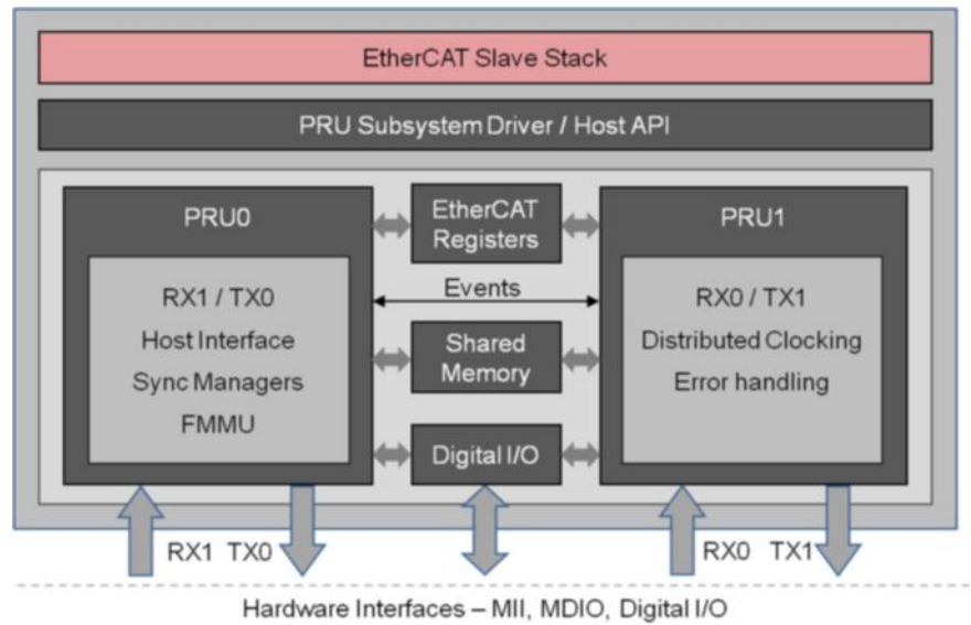
Figure 11. EtherCAT firmware architecture
